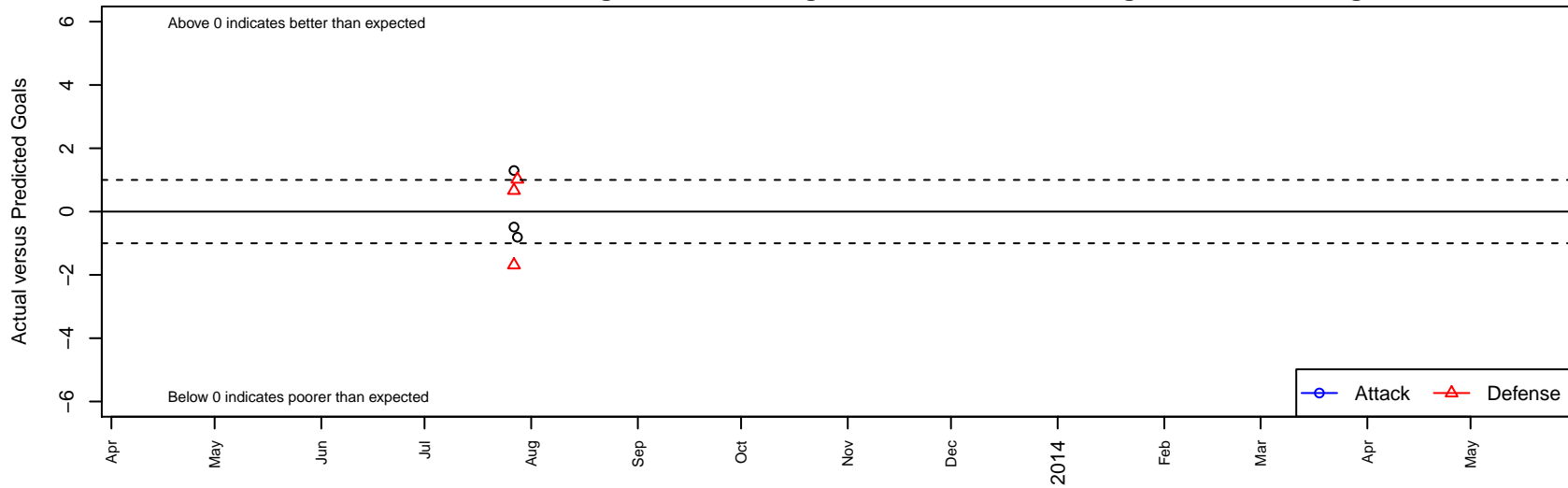
Bethesda SC Revolution B95 Dots are actual minus expected GF (blue circles) and GA (red triangles). Blue line is smoothed change in attack strength. Red is smoothed change in defense strength.
